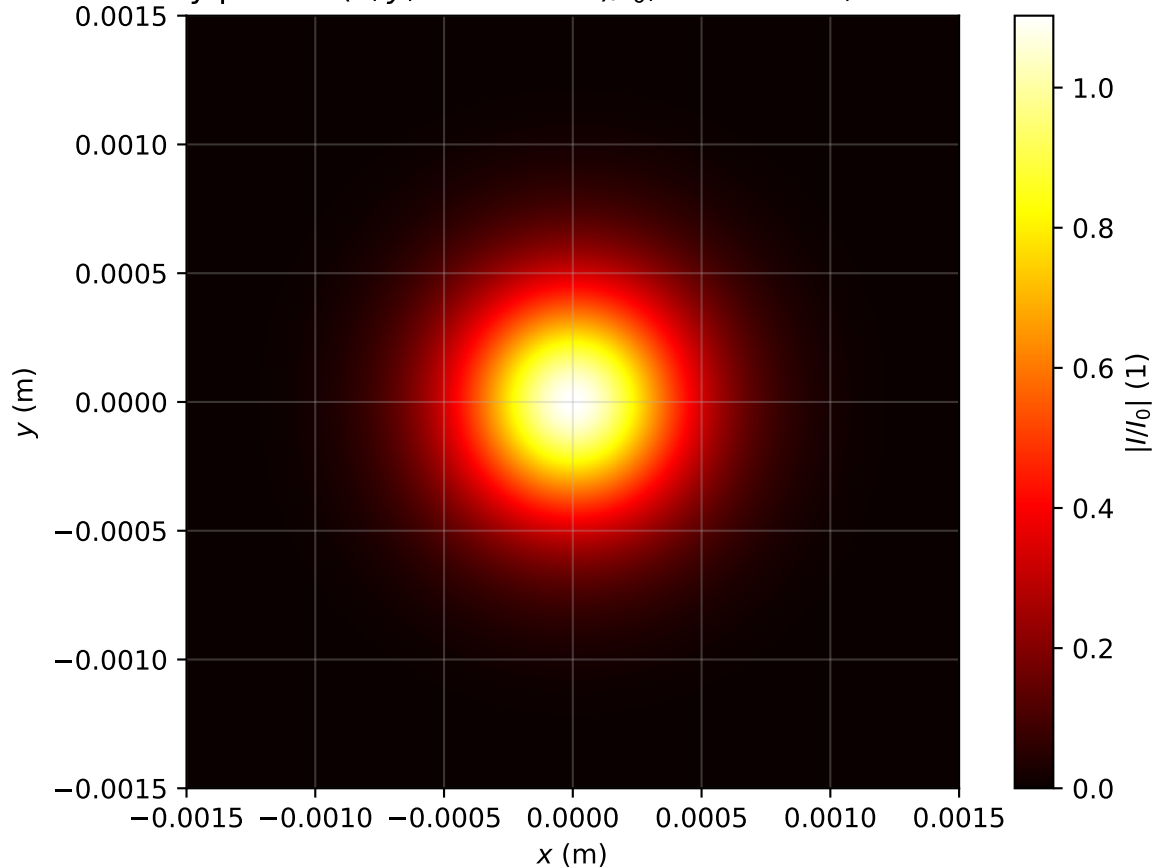
Intensity profile I(x, y, z = 0.716m)/I_0 , Pin=0.6Pcr, artificial time
